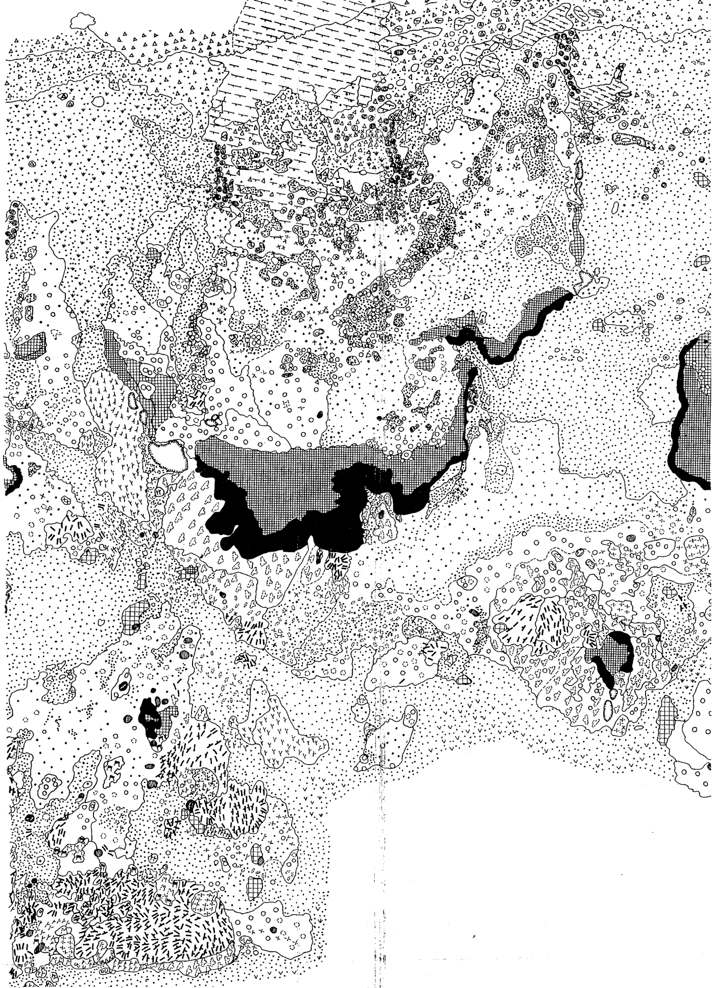
Fig. 36. Shark Reef. The largest and highest (17 cm) of the Boiler Bay ridges. A large cave occurs shoreward of the collapsed block at the east end of the reef. Sand Reef Skerry, offshore of Sand Reef is an A. palmata patch with 30-60 cm cap of coralline. For depths see figures 39 & 43A.
