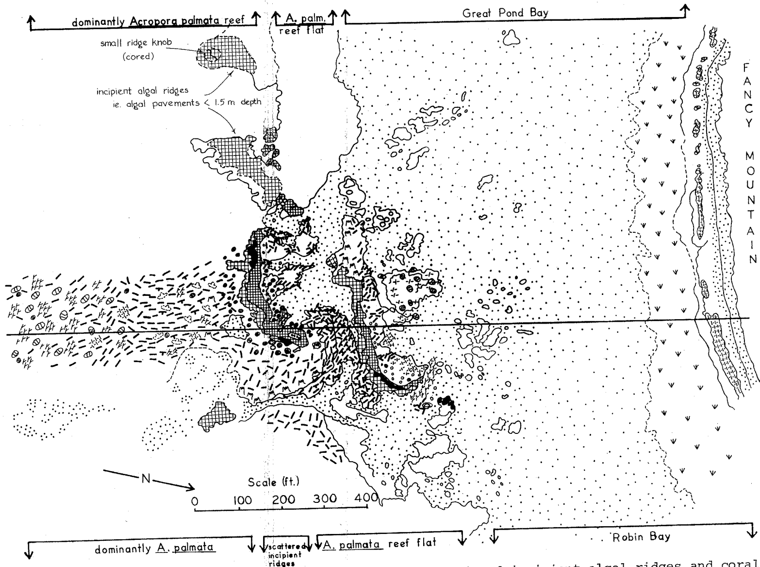
Fig. 22. Map of Fancy Mountain algal ridge pair and its associated incipient algal ridges and coral reef communities. Section shown in figure 23. ■ +15 to +30 cm above m.l.w.sp., ▨ -10 to +15 cm, ▩ -100 to -10 cm.
