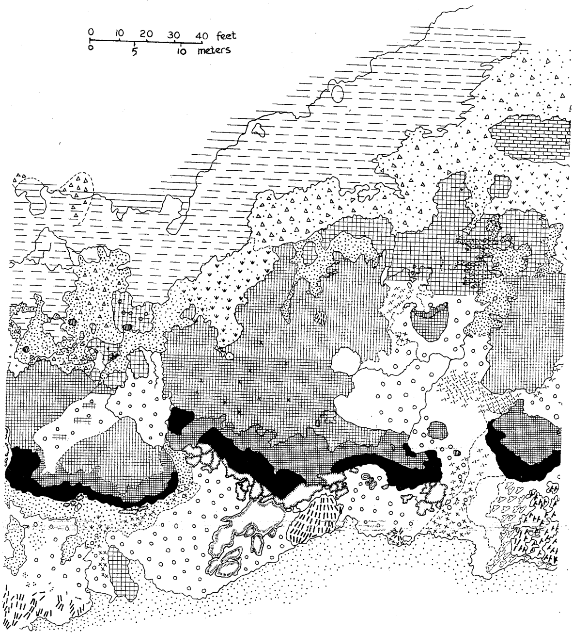
Fig. 33. Stick Reef and Breaker Reef. These are boiler-fused ridges, Stick Reef having some caverns, but the original boiler pattern is not obvious. Considerable collapse has occurred on the front of Breaker. See figure 41 for depths.
