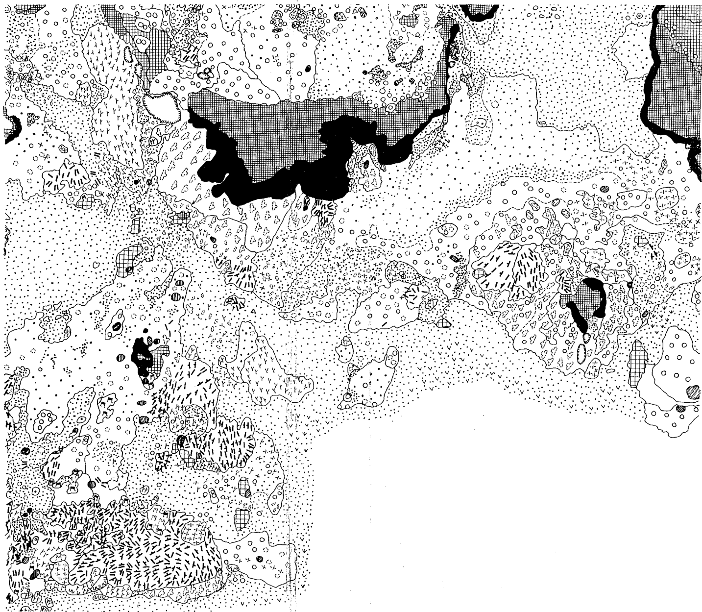
Fig. 36. Shark Reef. The largest and highest (17 cm) of the Boiler Bay ridges. A large cave occurs shoreward of the collapsed block at the east end of the reef. Sand Reef Skerry, offshore of Sand Reef is an A. palmata patch with a 30-60 cm cap of coralline. For depths see figures 39 & 43A.
