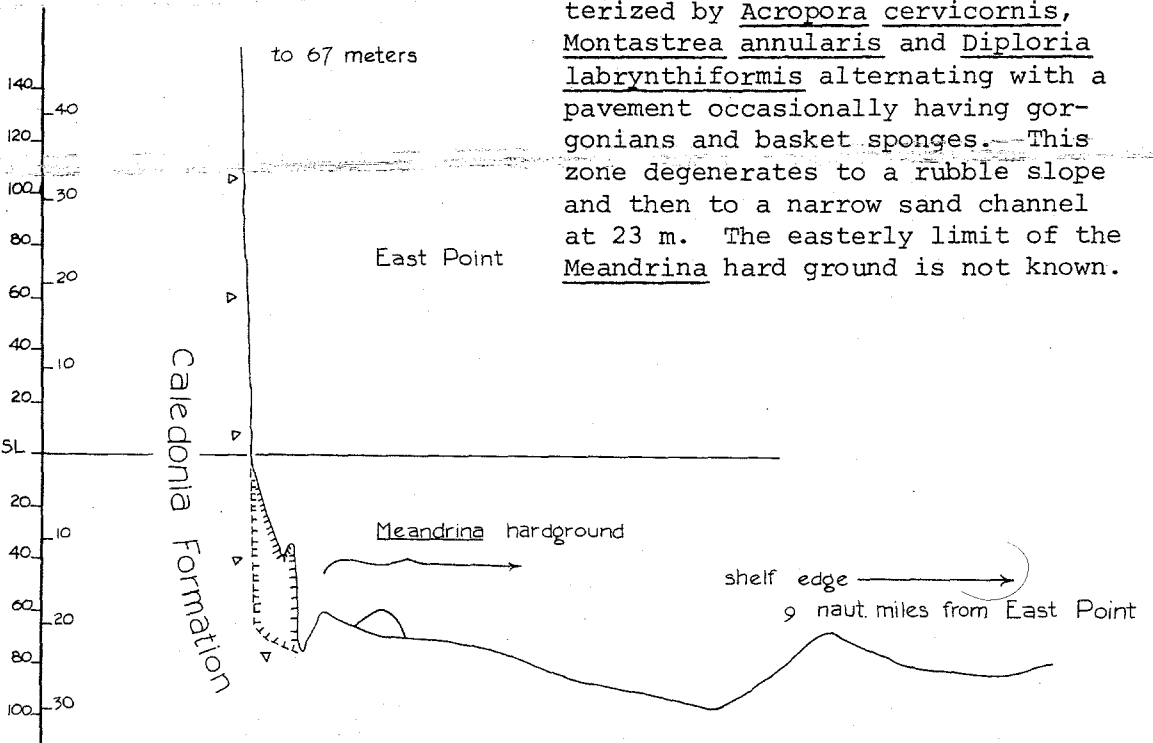
Fig. 9. Section through reef at East Point (Fig. 4). Basement depth estimated from previous sections. From -2 to -13 m, the reef is dominated by Acropora palmata on undercut blocks of A. palmata pavement separated by rubble-filled grooves and basins. A narrow rubble-sand band with gorgonians occurs at -13 m. The rather narrow deep fore-reef is characterized by Acropora cervicornis , Montastrea annularis and Diploria labyrinthiformis alternating with a pavement occasionally having gorgonians and basket sponges. This zone degenerates to a rubble slope and then to a narrow sand channel at 23 m. The easterly limit of the Meandrina hard ground is not known.
