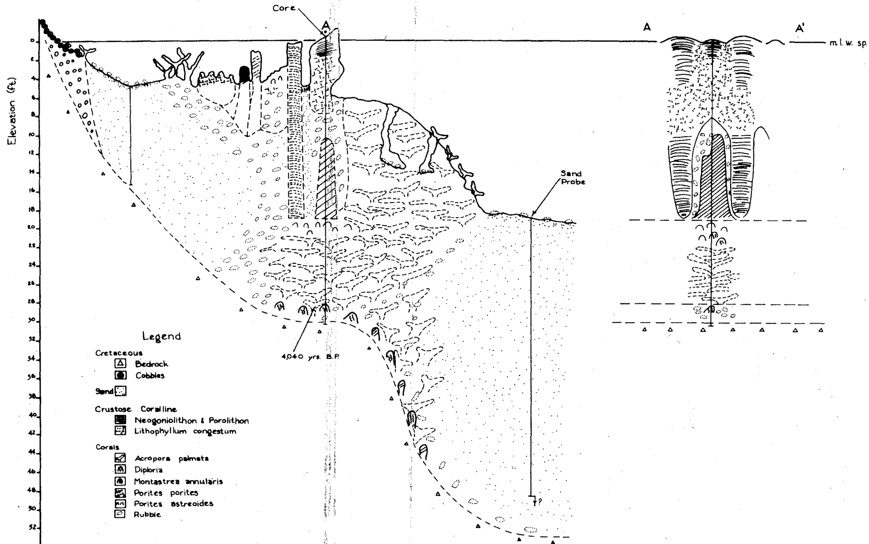
Fig. 21. Sections across Isaac Algal Ridge as shown in Figure 20. In the cores ▩ Lpm. congestum , ▨ crust corallines, ▣ coral rubble. The section AA' is an interpretation based on the surface characteristics of the boilers making up this section of the reef.
