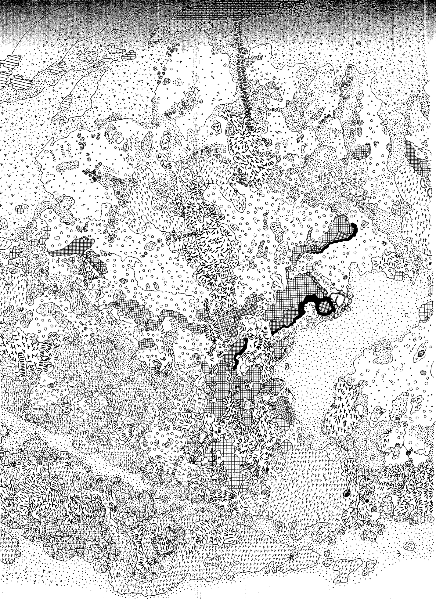
37. East Reefs. This partly fused complex of boilers began to degenerate before completion of ridge formation. For depths see figure 42A.
