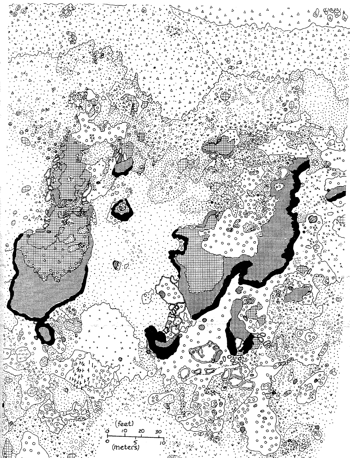
Fig. 35. Sand and Reference Reef algal ridges. Both of these are complexes of fused boilers. The outer end of the main section of Sand Reef is a 1-2 m overhanging lip. This joins the small offlying boiler to form a short tunnel. Considerable roof collapse has occurred on the outer part of Reference Reef. For depths see Fig. 42B.
