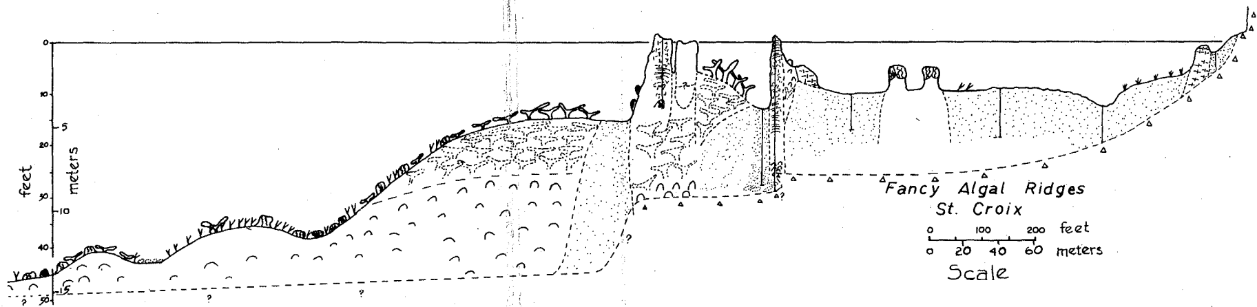
Fig. 23. Section from shore at Fancy Mountain, across Fancy algal ridges to the outer shelf. Symbols as previous figures. n inferred head corals Diploria spp. and Montastrea annularis .
