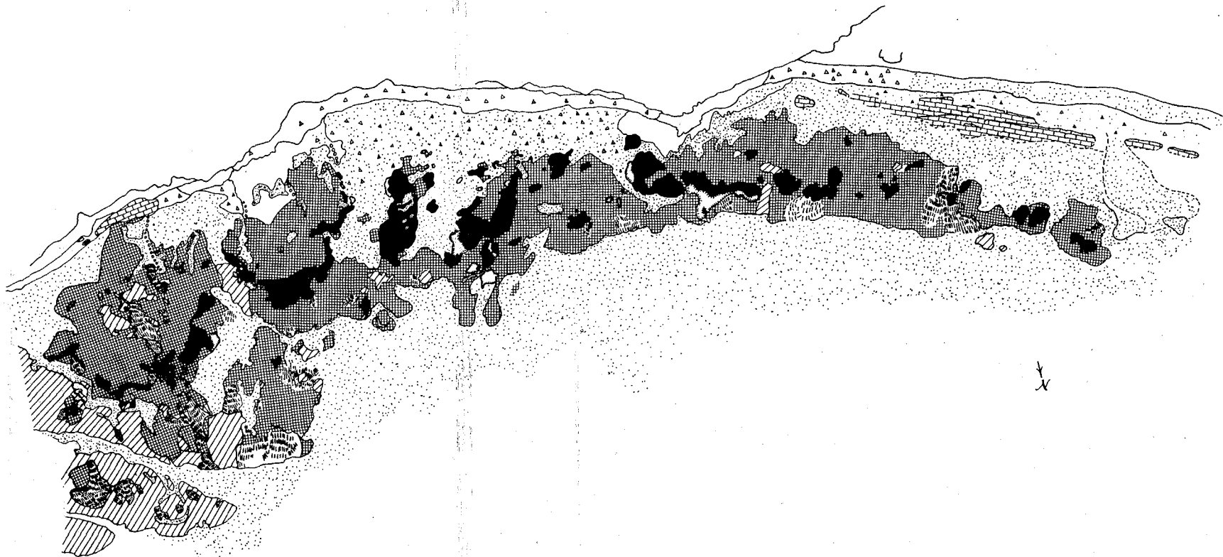
Fig. 45. Generalized surface structure of algal ridge area in Boiler Bay. ■ coralline-constructed algal ridges; ▣ coral pavements, mostly Porites porites and Acropora cervicornis (small variety), some A. palmata ; ▤ living A. palmata colonies; ▨ dominantly live coral, mostly P. porites and A. cervicornis areas.
